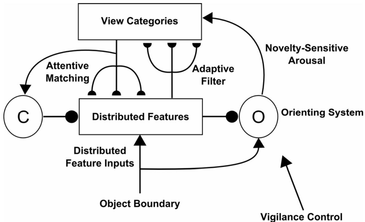
Figure 3. View category learning circuit. Top-down expectations are attentively matched against bottom-up input features. Attended critical features are learned. A big enough mismatch (i.e., one that does not satisfy the vigilance criterion in the orienting system O) causes a burst of novelty-sensitive arousal from O that inhibits the active category and triggers search for and learning of a better matching category. C: biased competition; black arrowheads: excitatory connections; black disks: inhibitory connections; black semi-circles: learned connections.
