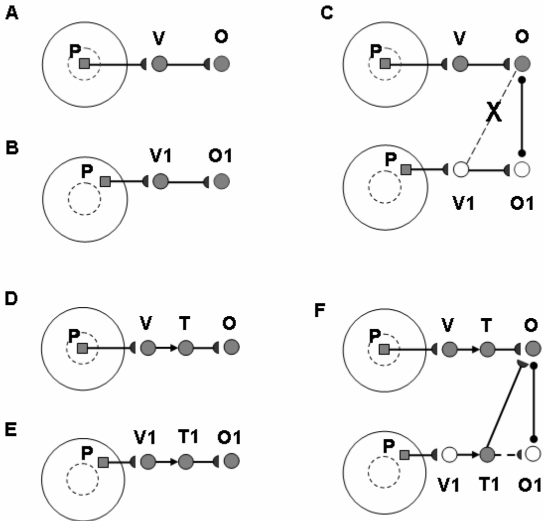
Figure 4. How view category integrator neurons help to learn spatially-invariant object categories. Large circles denote retinas; dotted circles denote foveas within the retinas; filled little squares denote object retinal images; filled little circles denote active neurons; open little circles denote inactive neurons; lines with black disks denote inhibitory connections; black semi-circles denote learned connections; black arrowheads denote excitatory unlearned connections; dotted line with X denotes no learned connection can occur; dotted line with semi-circle denotes losing learned connection. See text for details.
