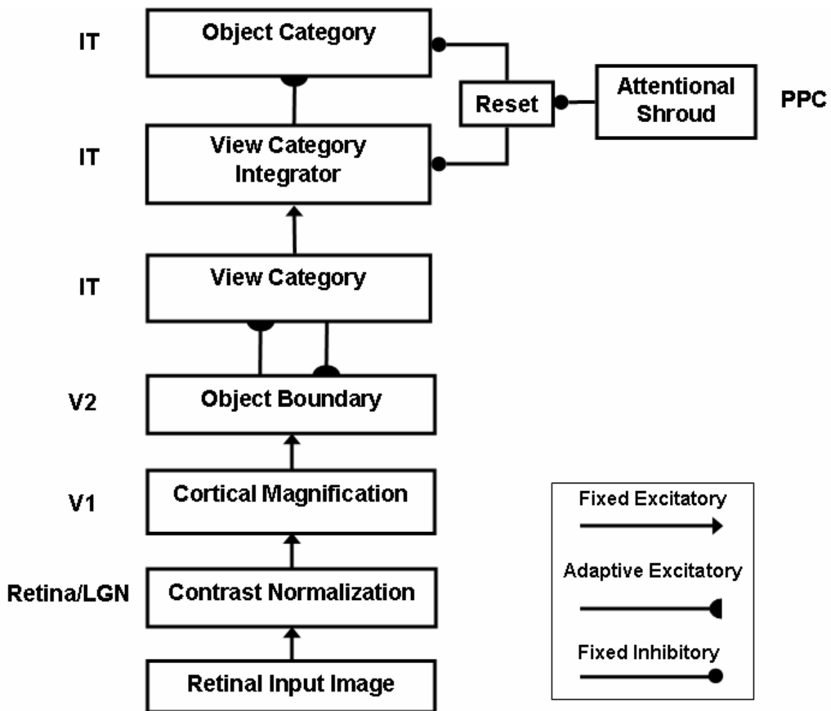
Figure 2. Model processing stages. See text for details.
