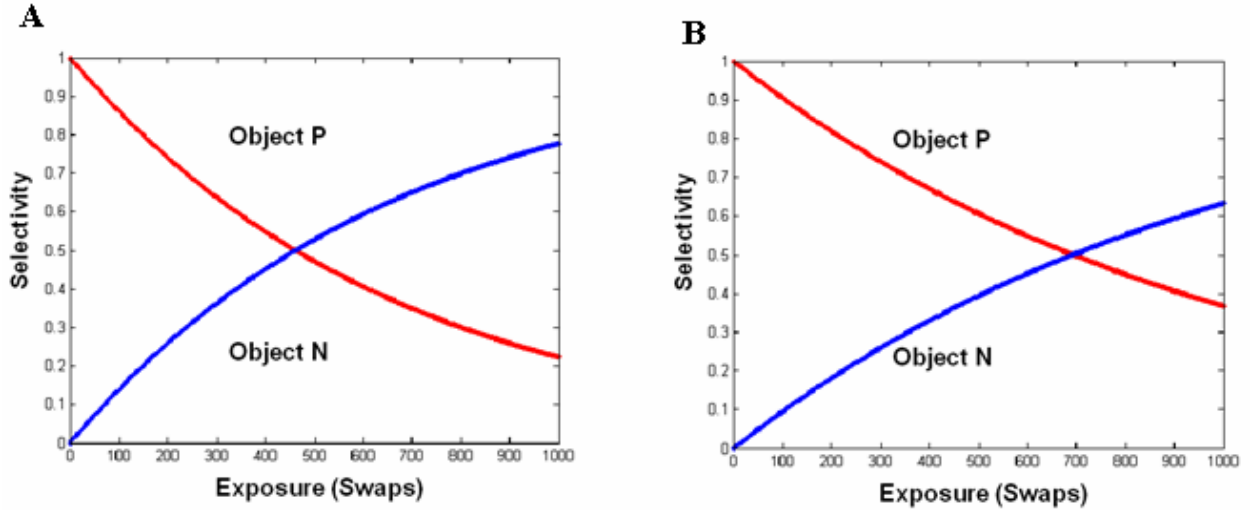
Figure 7. Model Simulations when the learning rate \alpha in (24) varies. (A) Increasing the learning rate to \alpha = 0.006 advances the selectivity reversal time. The selectivity of model IT object category neuron O_p to views of objects P and N at swap position reverses at about 450 swaps. (B) Decreasing the learning rate to \alpha = 0.004 delays the selectivity reversal time. The selectivity reverses at about 700 swaps now.
